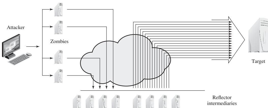
Figure 7.7 Amplification Attack
