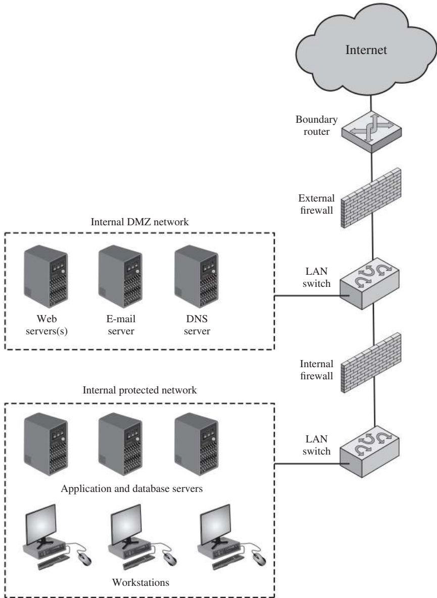
Figure 9.2 Example Firewall Configuration
