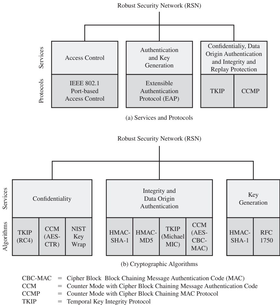
Figure 24.6 Elements of IEEE 802.11i
