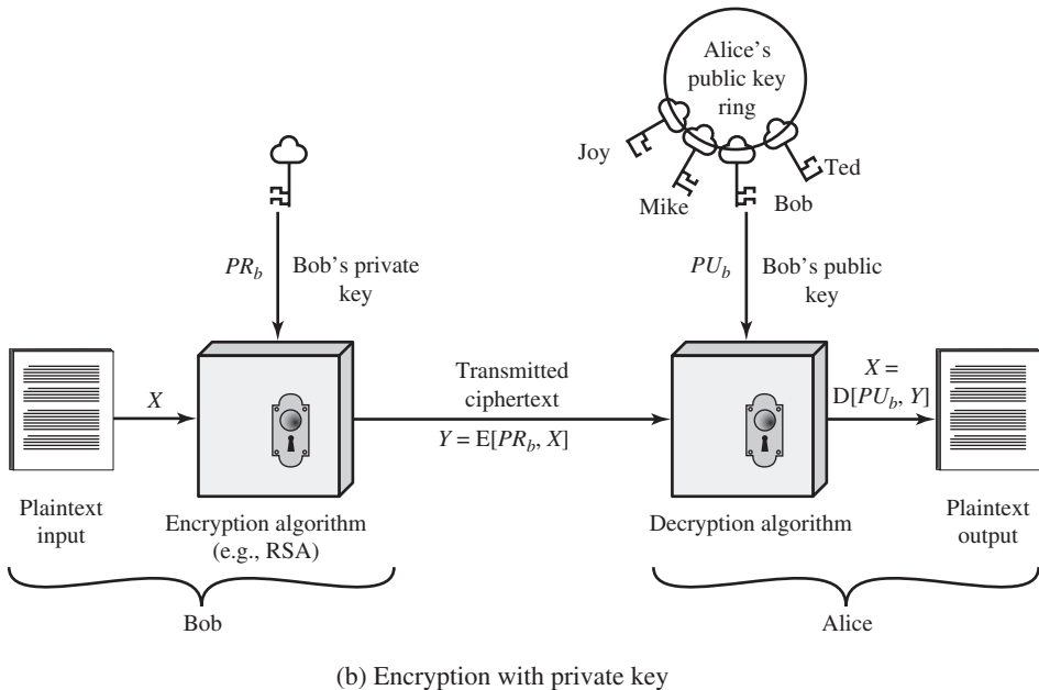
Figure 2.6 Public-Key Cryptography
