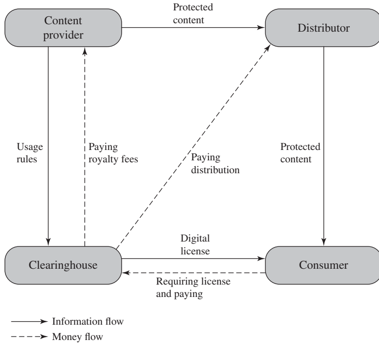
Figure 19.2 DRM Components
