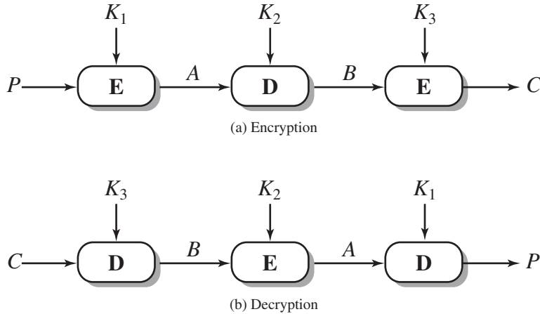
Figure 20.2 Triple DES
