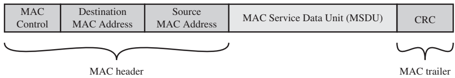
Figure 24.4 General IEEE 802 MPDU Format
