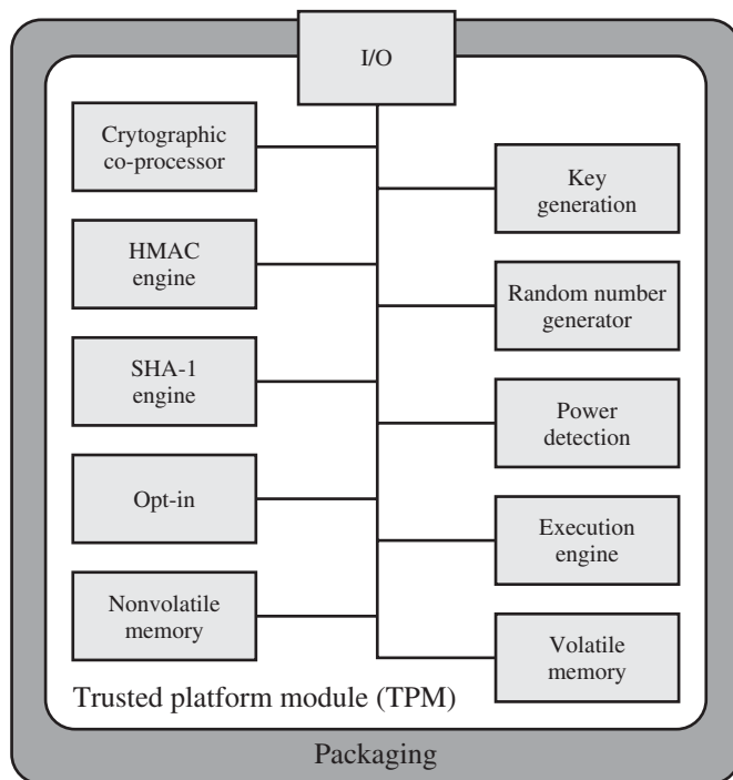
Figure 13.11 TPM Component Architecture
