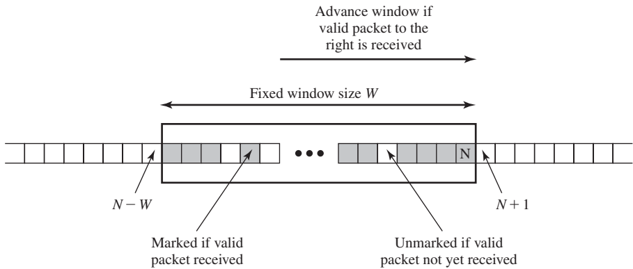
Figure 22.9 Antireplay Mechanism
