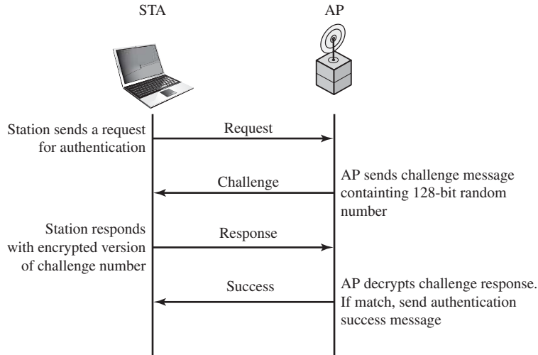
Figure 24.13 WEP Authentication
