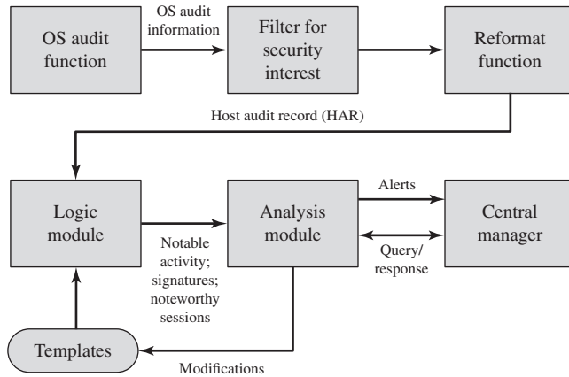
Figure 8.3 Agent Architecture
